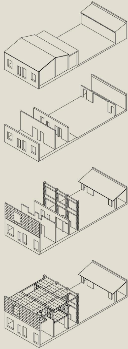
Axonometric View
