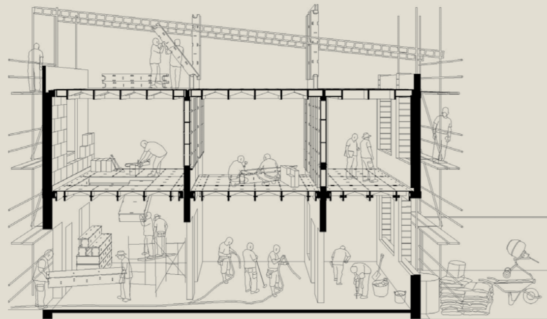
Perspective Section
