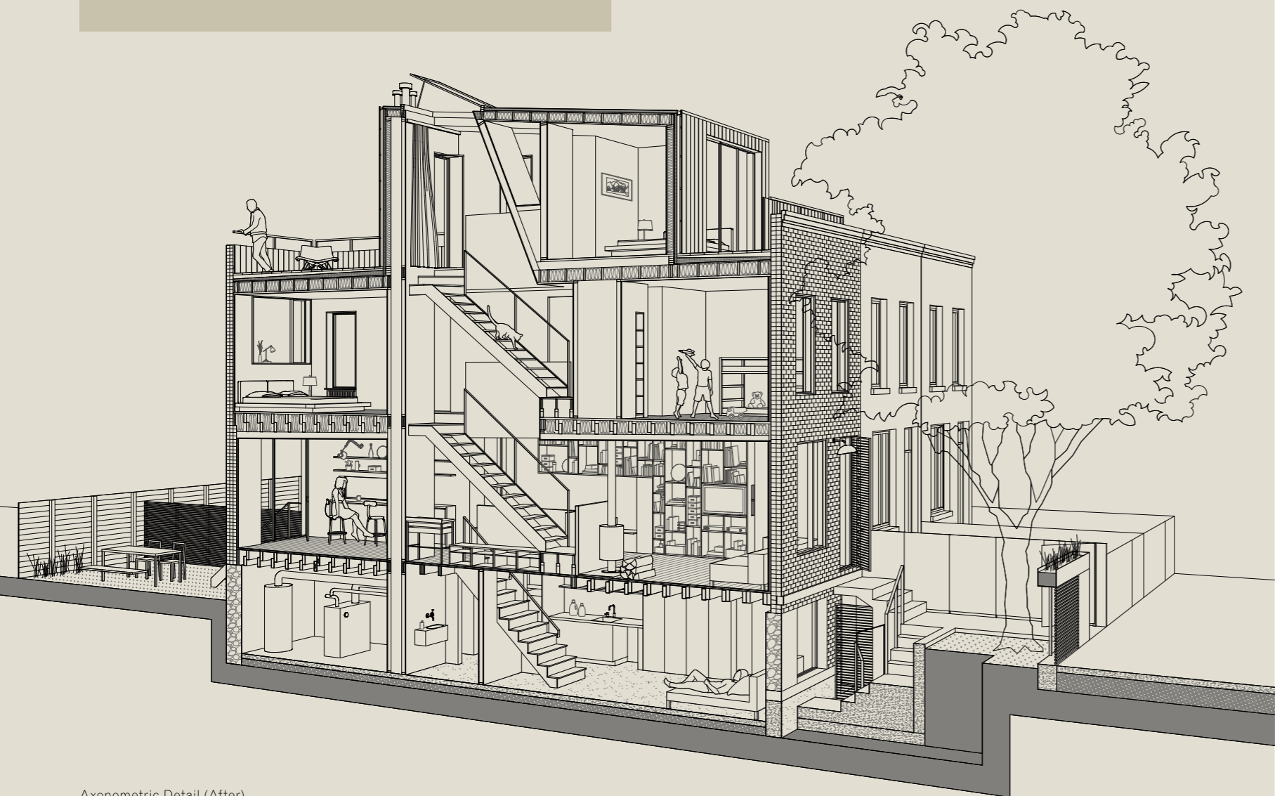
Axonometric Detail (After)
